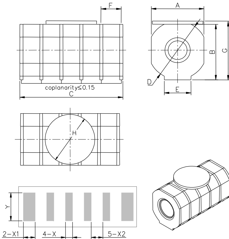
Recommended Soldering Pad Layout
